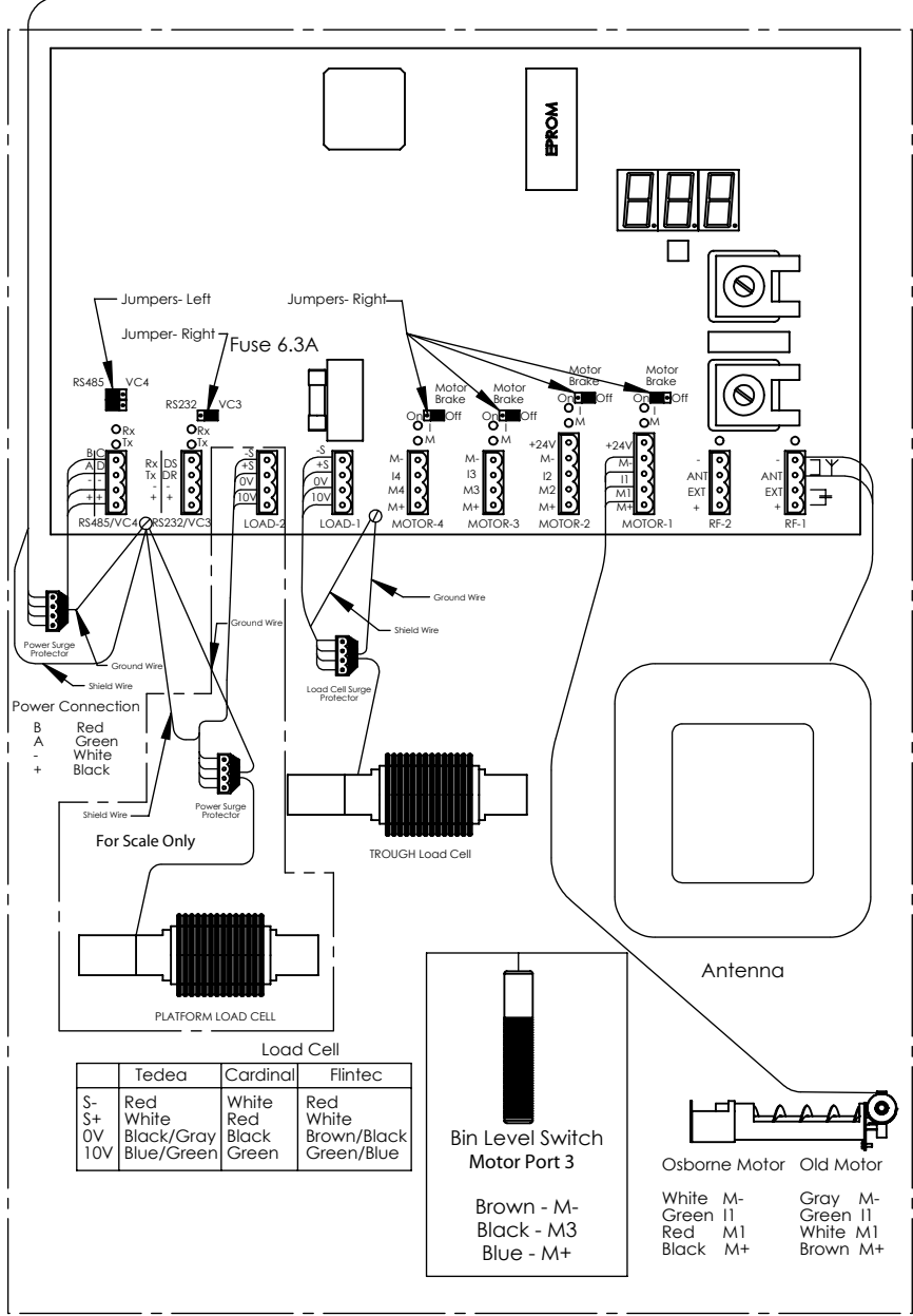
DETAIL C
